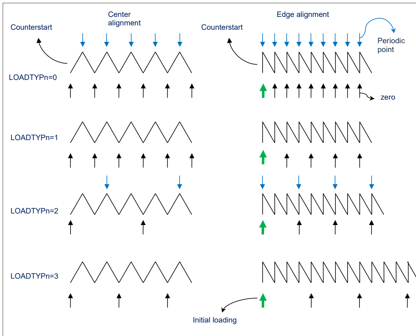
Figure 16-2: PWM period/duty cycle loading update block diagram
