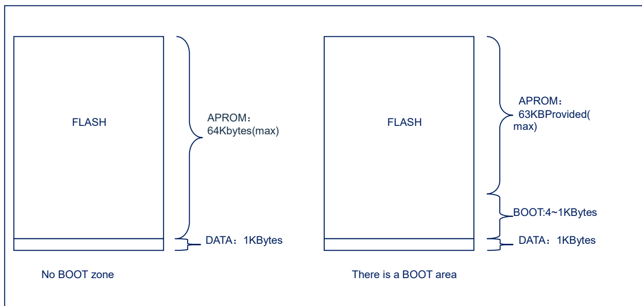
Figure 25-1: Storage structure diagram
